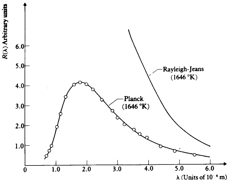
1.5 The Rayleigh-Jeans and Planck distributions at 1646 K. The dots represent the experimental points of Lummer and Pringsheim.
